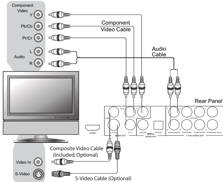
Method 3 – Component Video Connection to TV
